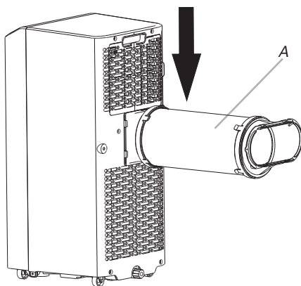
A. Flexible exhaust hose assembly
