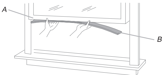
A. Lower window sash B. Adhesive seal
